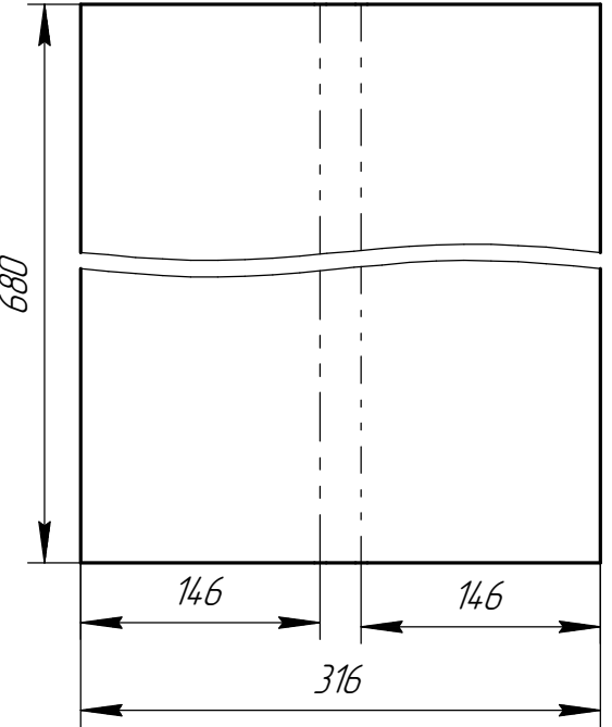
Q (1:5)
